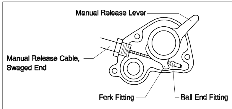
Figure 2-2 Manual Release Cable Rig
