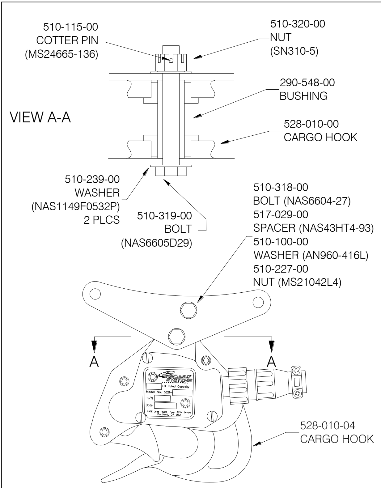
Figure 2-1 Attach Hardware Installation
