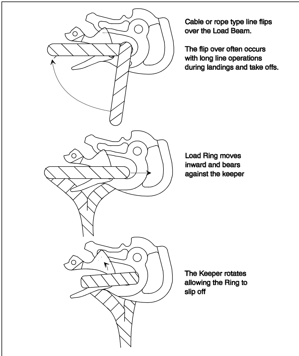
Figure 5 Un-commanded release due to cable or rope type straps
