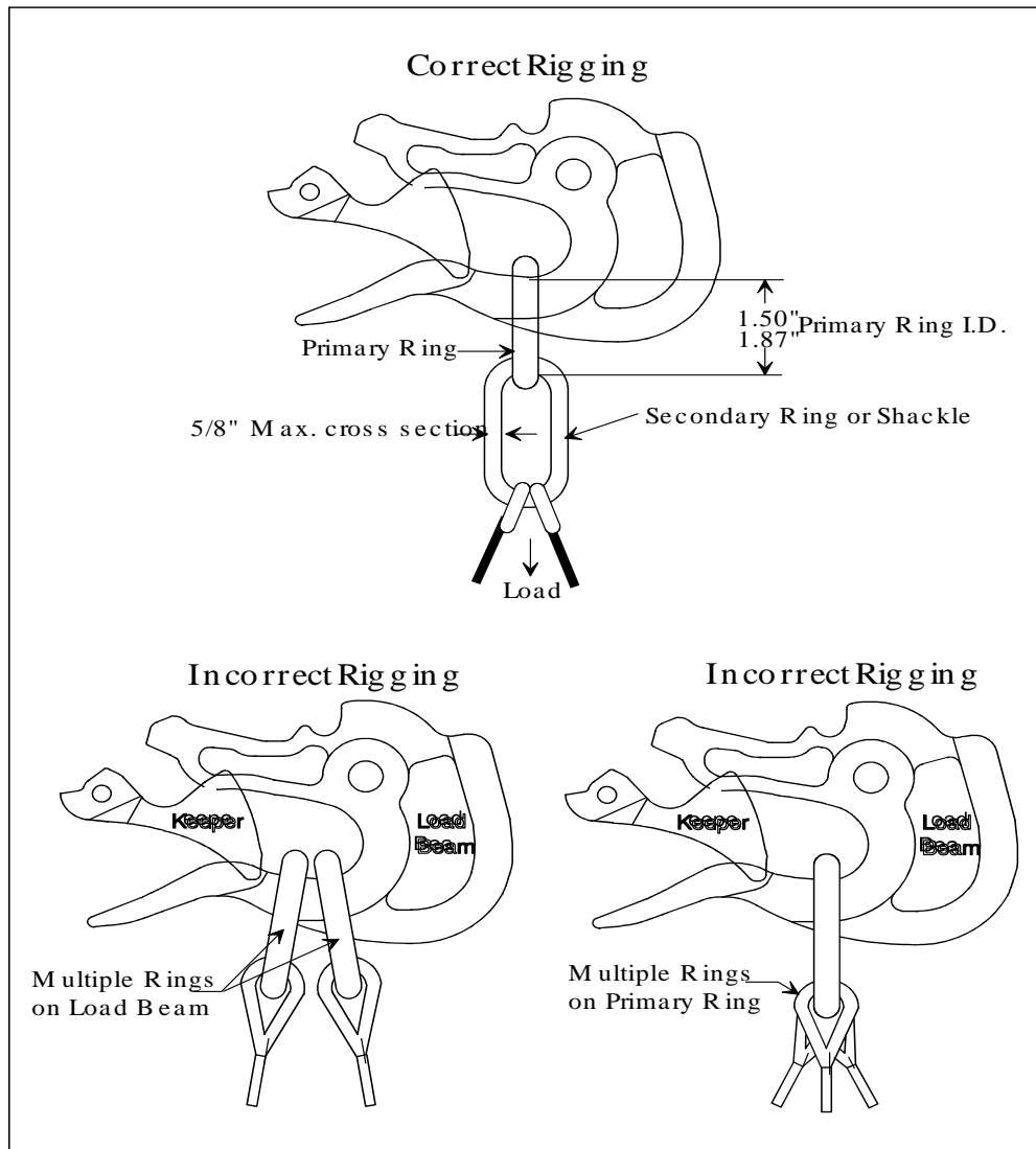
Figure 1 Examples of correct and incorrect cargo hook rigging
