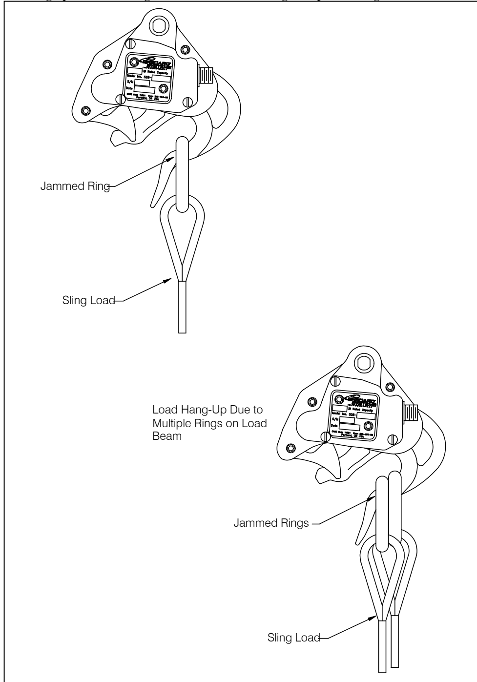
Figure 3 Load hang-up due to load rings that are too small or using multiple load rings
