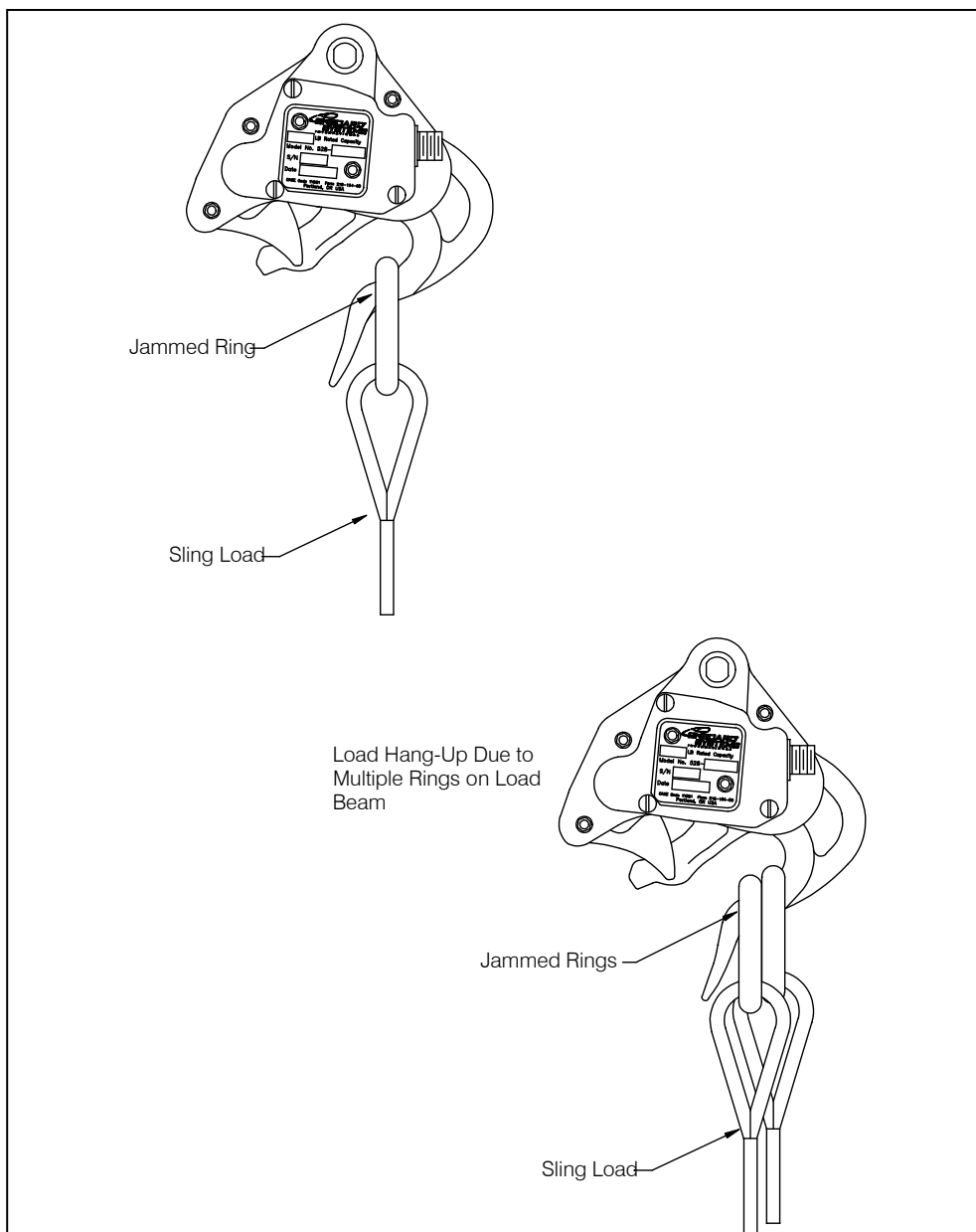
Figure 3-3 Load Hang-Up Due to Too Small a Load Ring or Multiple Load Rings
