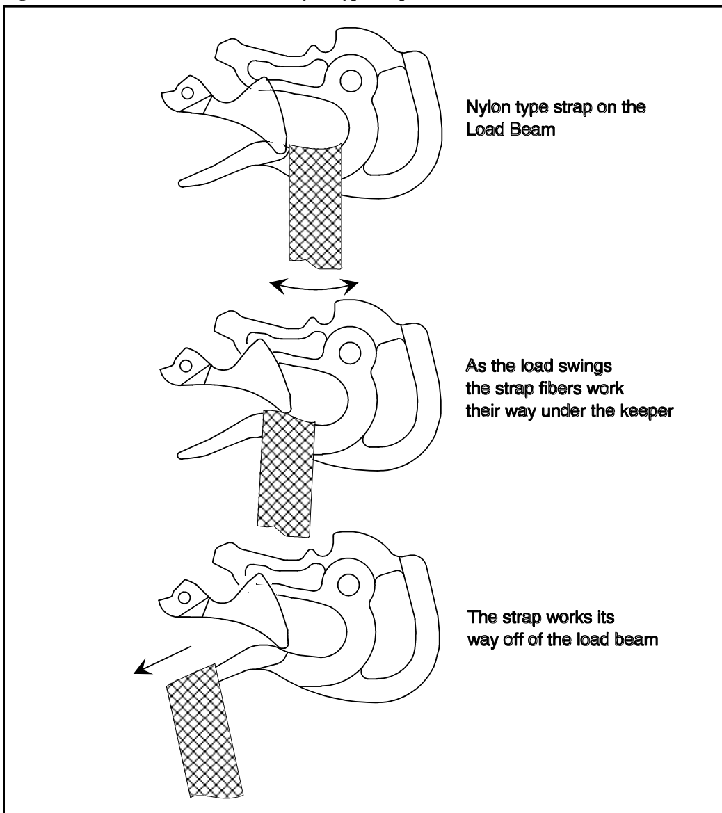
Figure 4 Un-commanded release due to nylon type straps
