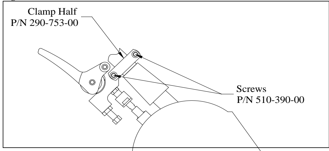
Figure 2.1.2 Manual Release Lever Installation
