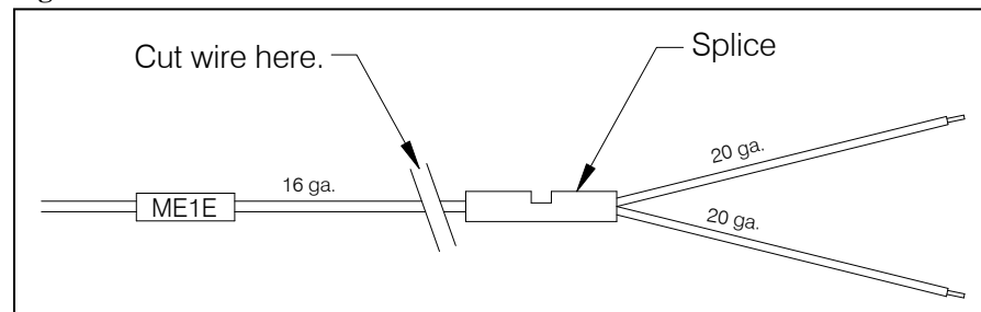
Figure 2.3.2 P/N 270-108-00 Harness Modification
