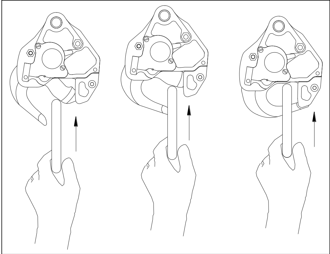
Figure 4.2 Cargo Hook Loading
