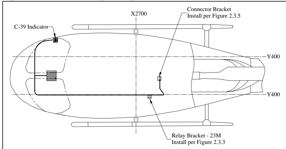
Figure 2.3.1 Electrical Wiring Routing Overview
