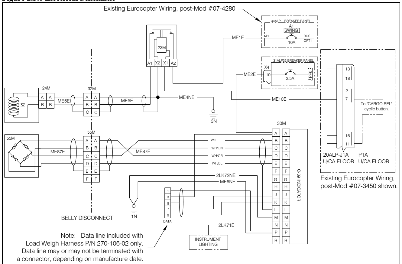
Figure 2.3.6 Electrical Schematic
