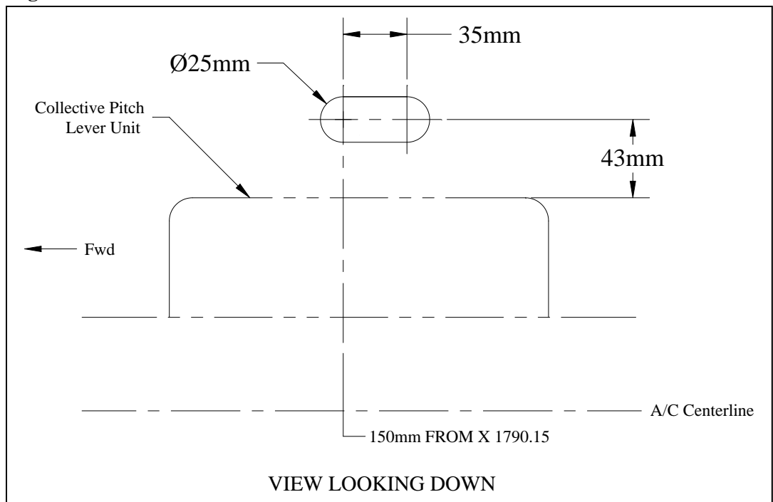
Figure 2.1.3 Cabin Floor Hole Detail
