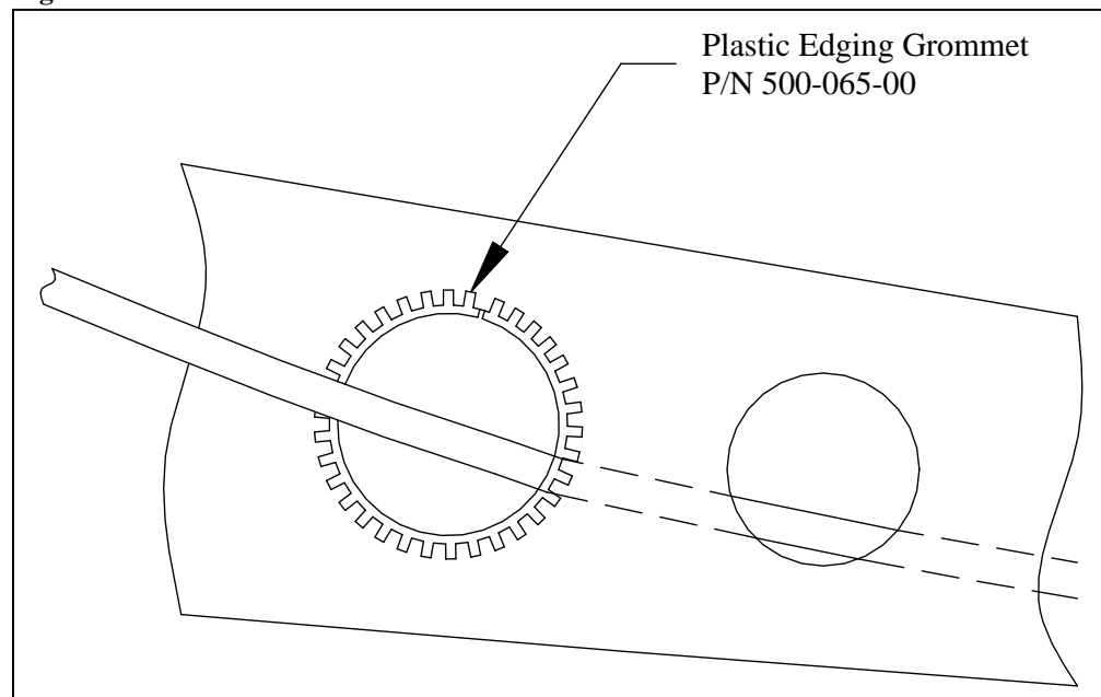
Figure 2.1.5 Grommet Installation
