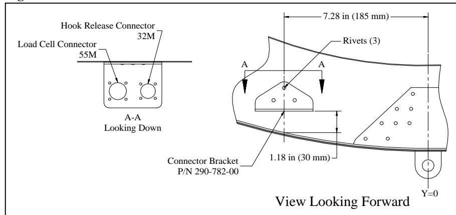
Figure 2.3.5 Connector Bracket Installation
