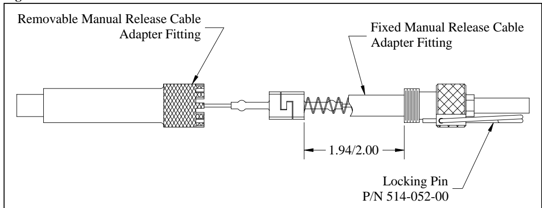
Figure 2.5.2 Manual Release Cable Connection
