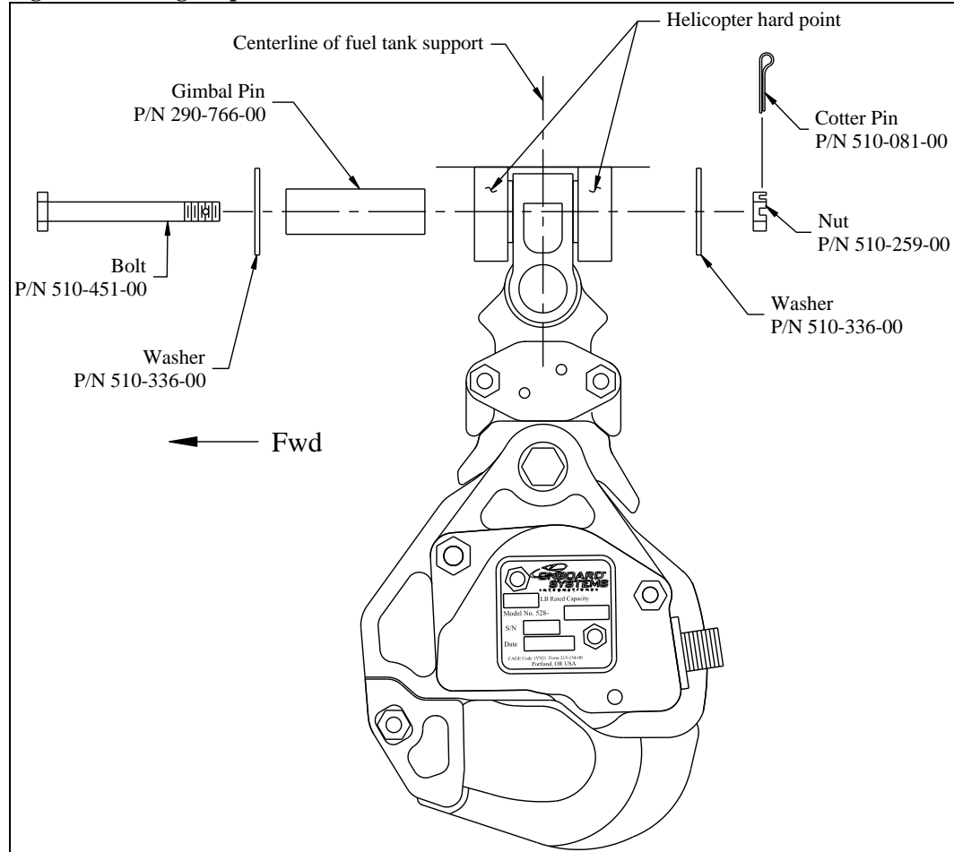
Figure 2.4.1 Sling Suspension Installation
