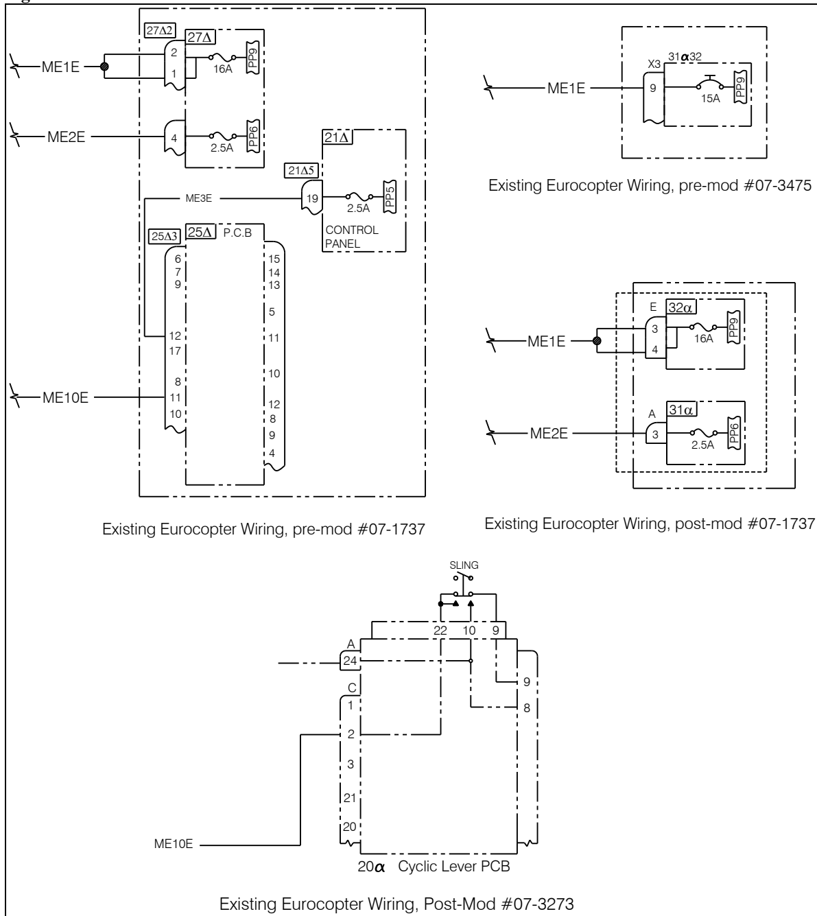
Figure 2.3.6 Electrical Schematic continued
