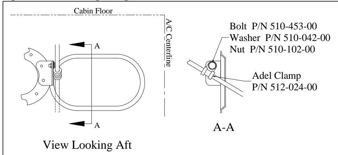
Figure 2.1.4 Cable Routing Through Frame
