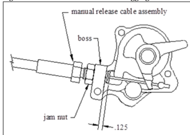
Figure 2.5.1 Manual Release Cable Rigging
