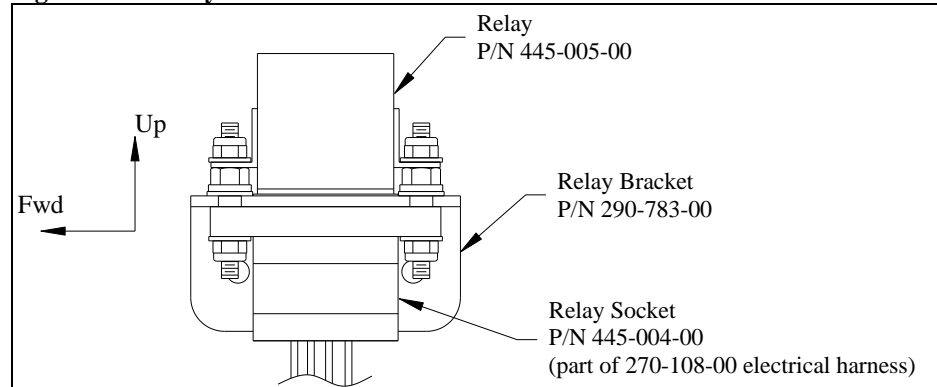
Figure 2.3.4 Relay Installation
