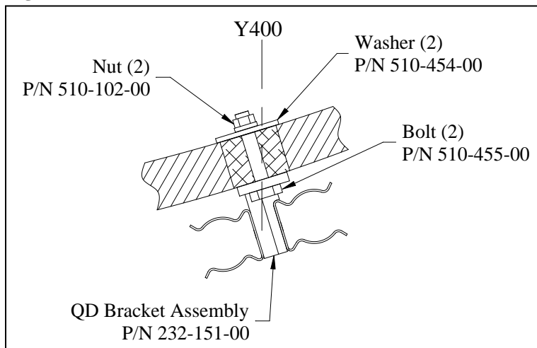
Figure 2.1.7 QD Bracket Installation
