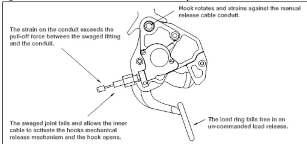
Figure 2.6.1 Un-commanded Release From Incorrectly Secured Cable
