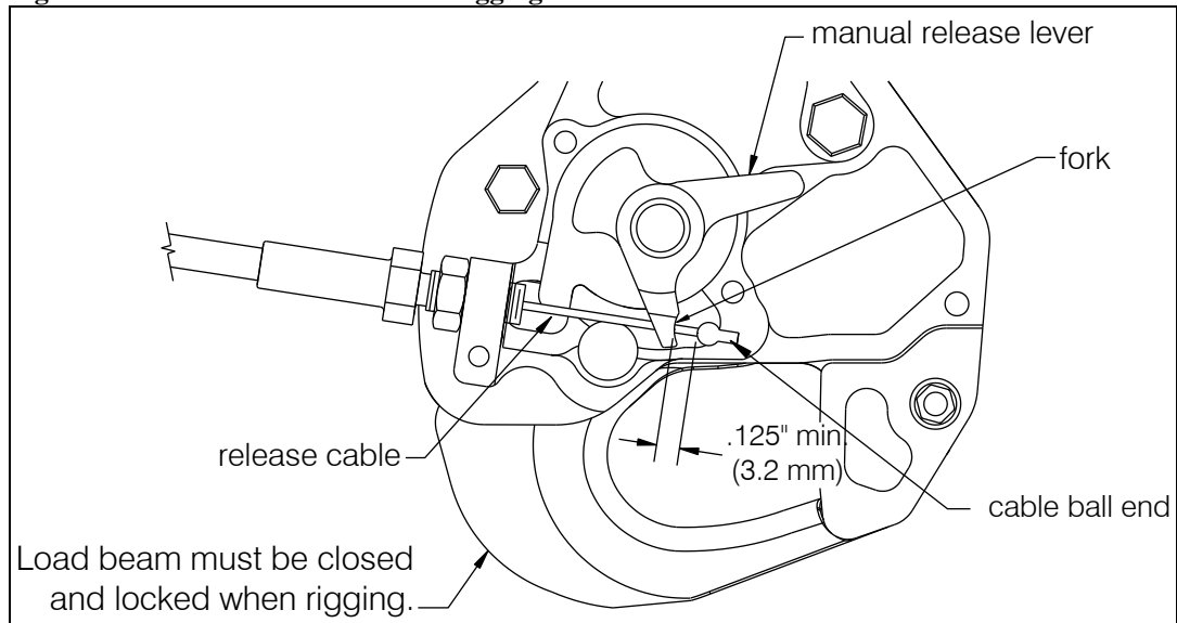
Figure 2.5.3 Manual Release Cable Rigging Check
