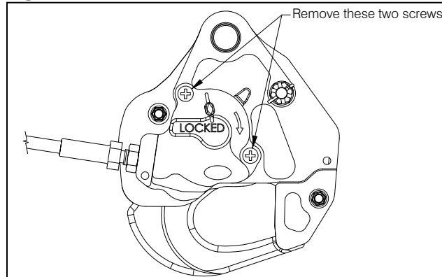
Figure 25.16.1 Manual Release Cover Removal
