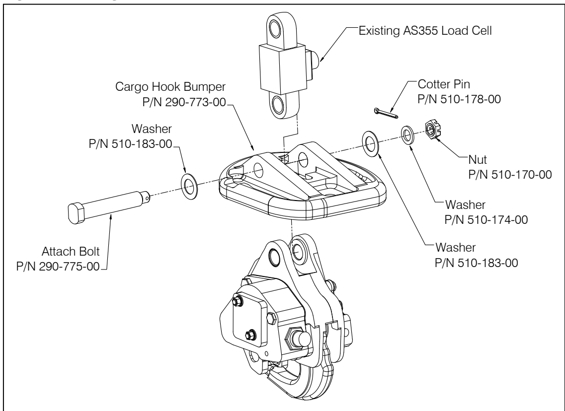
Figure 25.17.1 Cargo Hook Attachment Hardware
