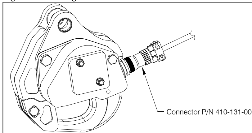
Figure 25.16.2 Cargo Hook Connector
