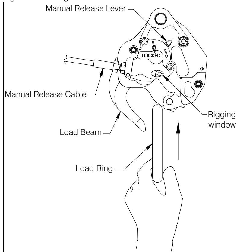
Figure 25.2.1 Cargo Hook Overview
