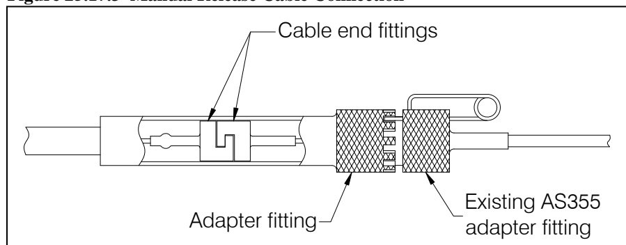
Figure 25.17.3 Manual Release Cable Connection
