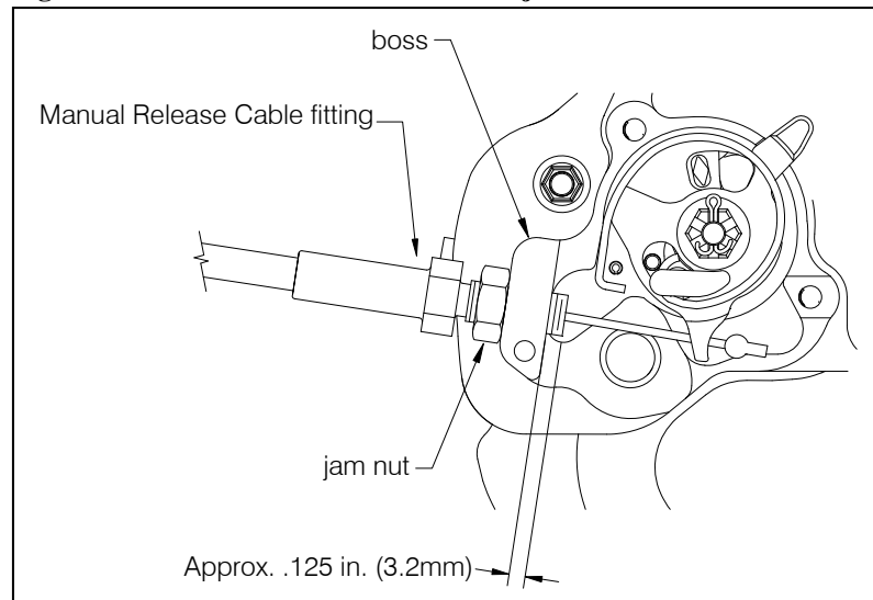
Figure 25.17.2 Manual Release Cable Adjustment
