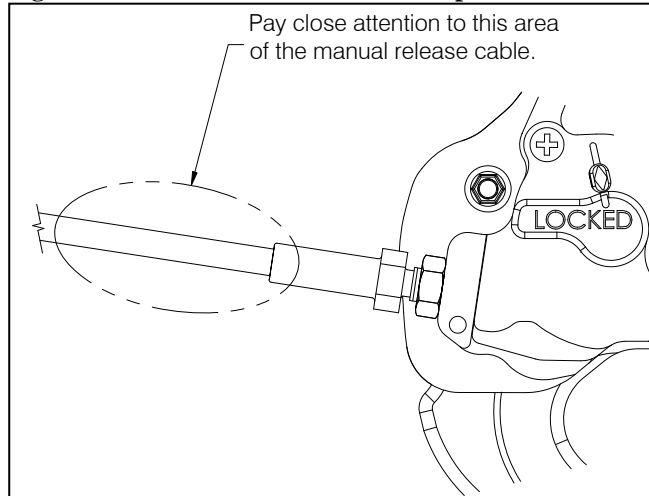
Figure 5.1.3 Manual Release Cable Inspection
